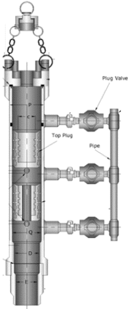
NON-QUICK LATCH TYPE (WITH DOUBLE PLUG)
