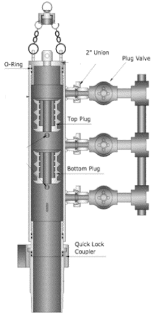
QUICK LATCH TYPE (WITH DOUBLE PLUG)
