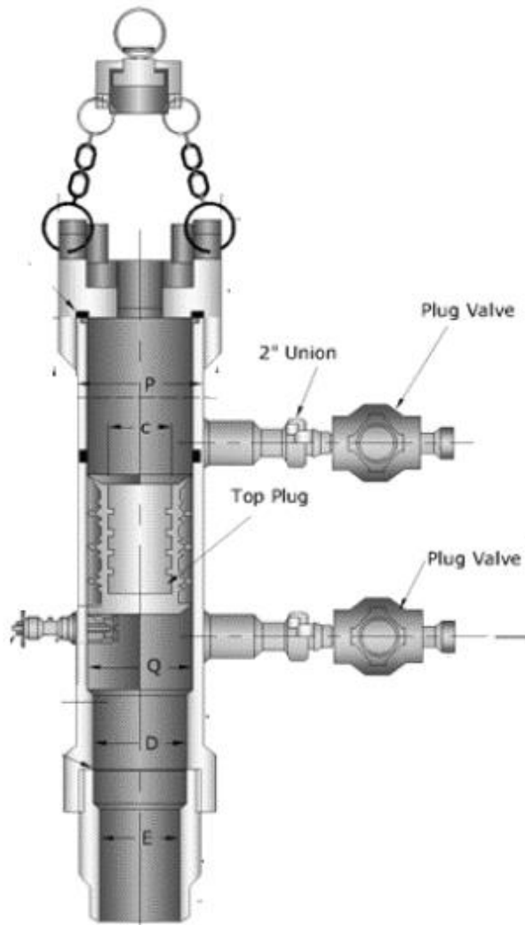
CASING CEMENTING HEAD (SINGLE PLUG)
